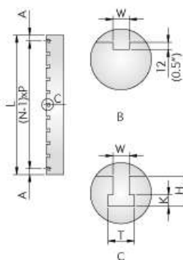
Without thermal compensation system
