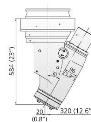
30° Angle Head (Manual Tool Release)
