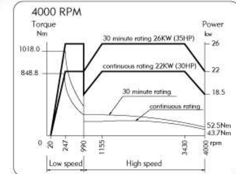
FANUC SPINDLE MOTOR: \alpha 22i, 22/26 KW (30 / 35 HP)
