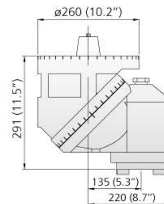
Universal Head Max. Speed: 1500 rpm
