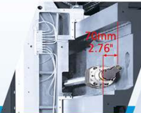
Y AXIS STEP DESIGN
